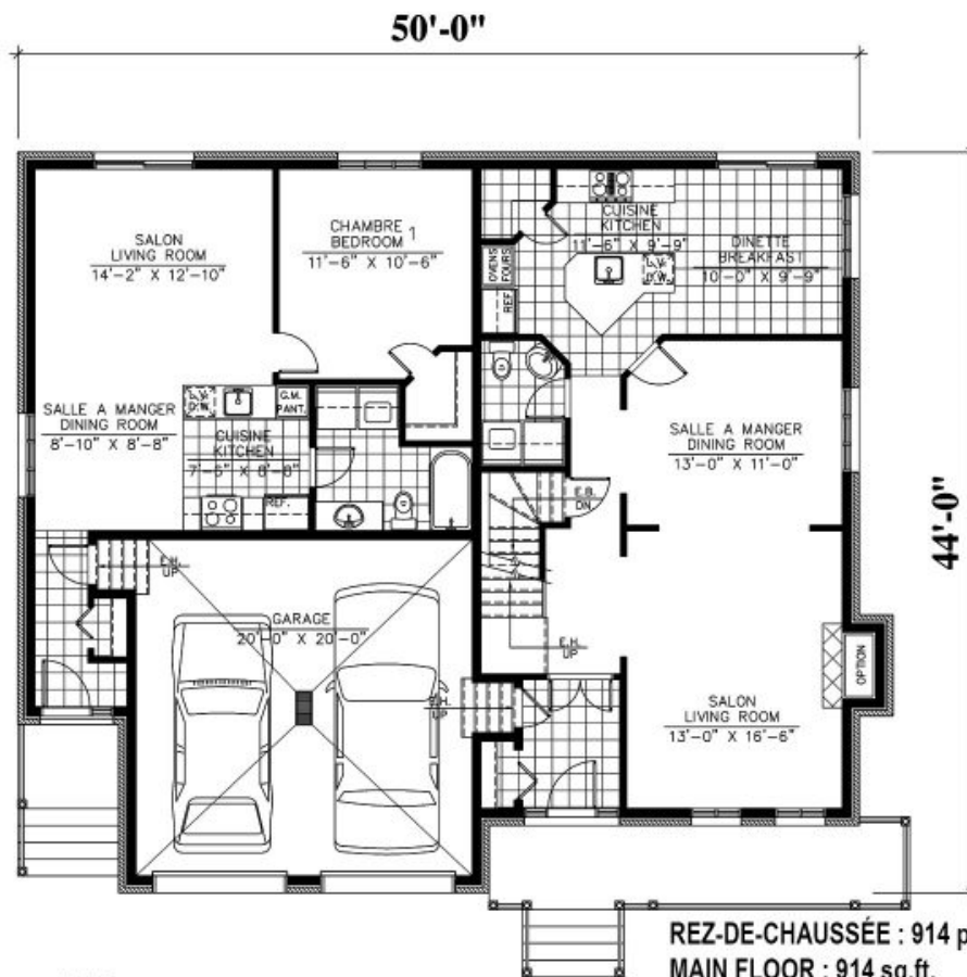
Plan Inversé / Reversed Plan # 416 - La Garonne
