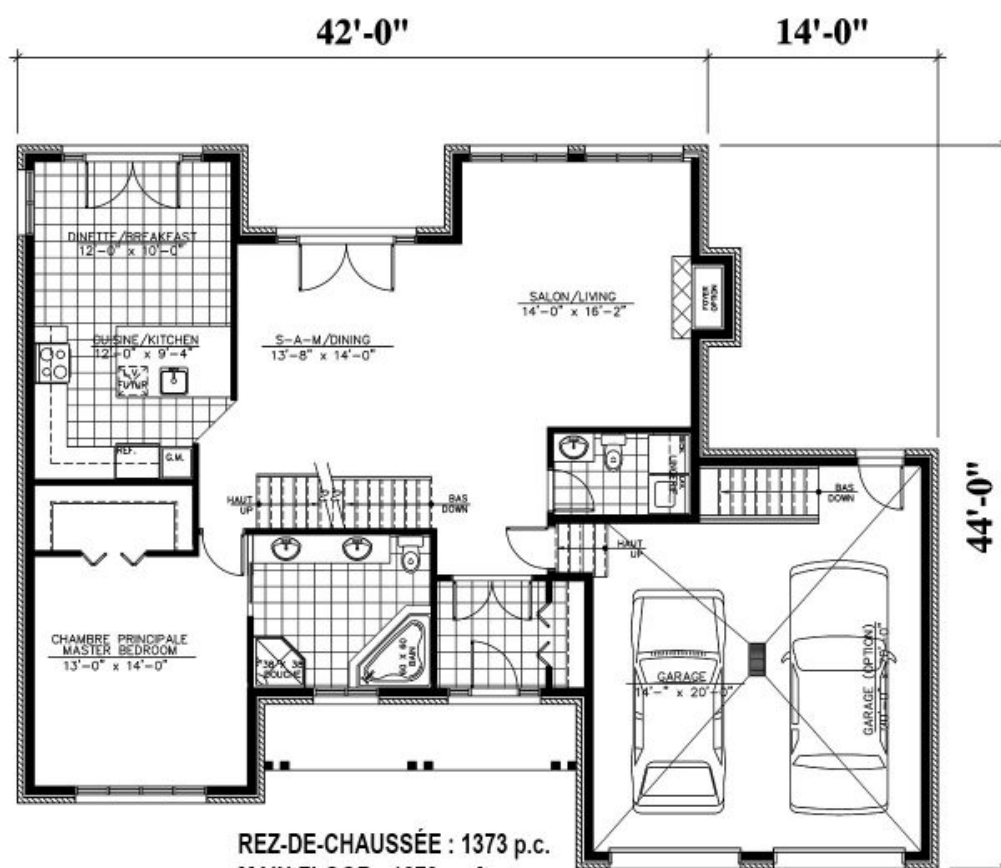
Plan Inversé / Reversed Plan # 444 - La Lyre
