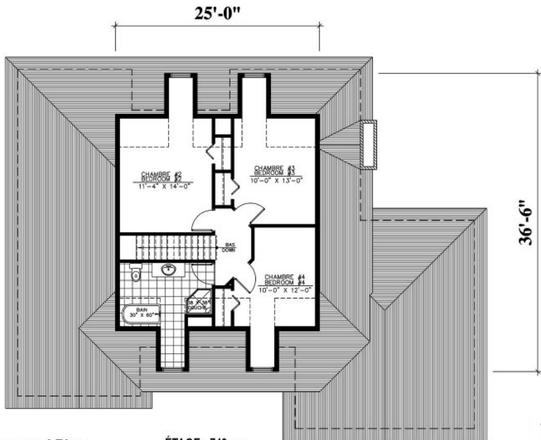
Plan Inversé / Reversed Plan # 444 - La Lyre
