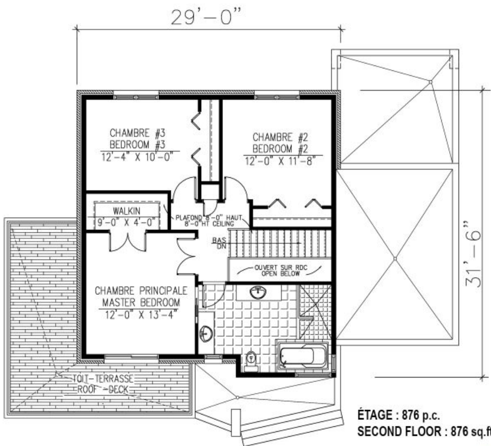
Plan Inversé / Reversed Plan
