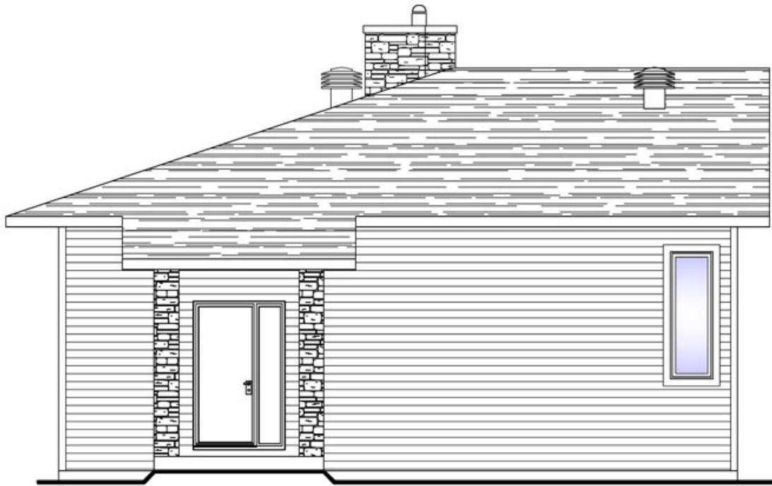
Façade
