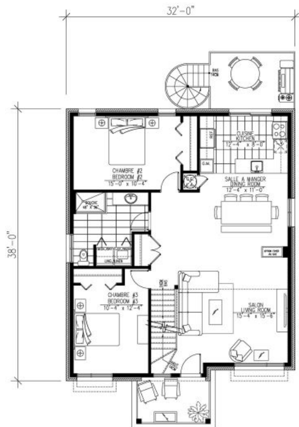
Plan Inversé / Reversed Plan
