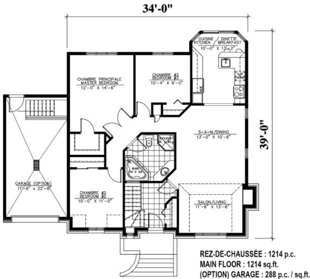
Plan Inversé / Reversed Plan
