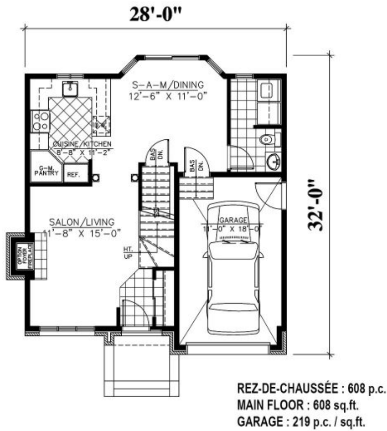
Plan Inversé / Reversed Plan
